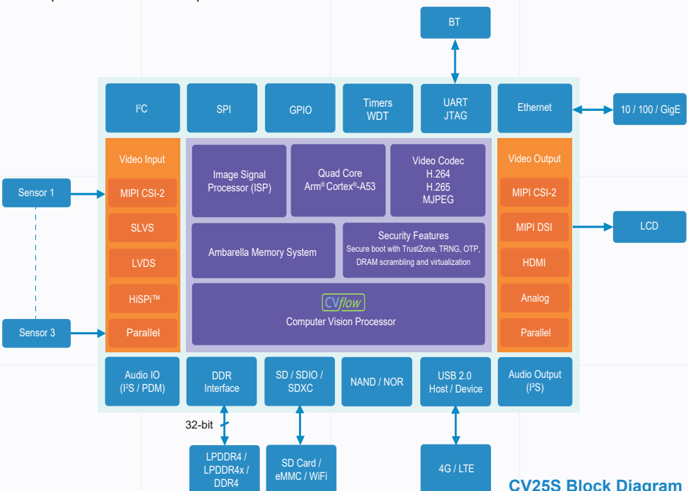
CV25S Block Diagram
