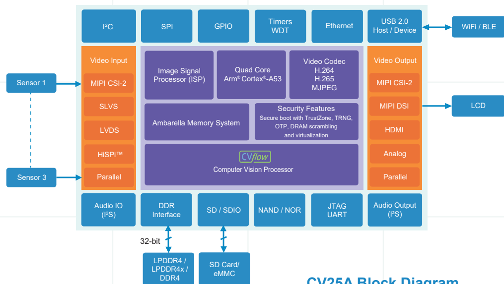
CV25A Block Diagram
